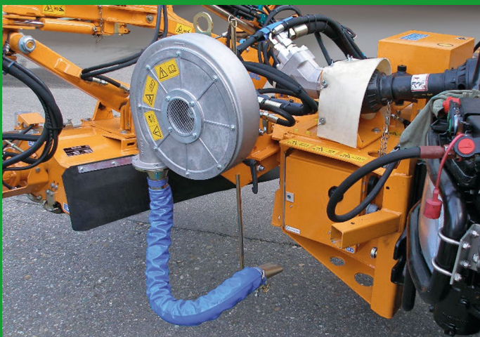
Optional pressure blowing system for effective road cleaning
