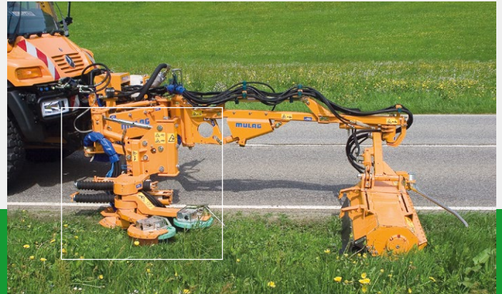
Easy extendible with a reflexion post mower MLM 200
