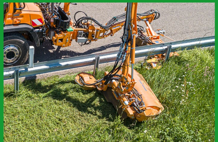
Combination use of the ZMS 400 additional mowing disc on the MKM 700
