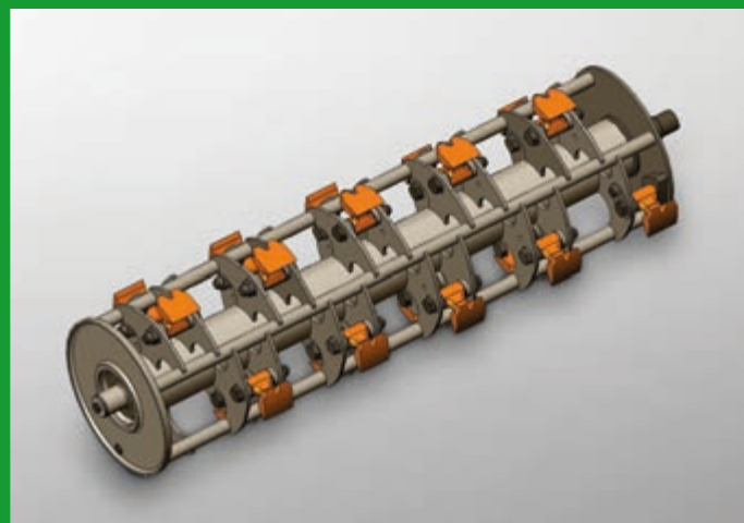
Schematic illustration of the GMK 1200 cutting shaft
